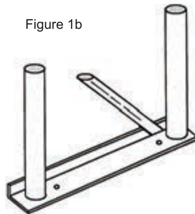
Figure 1b A continuous bearing plate joining the two posts
